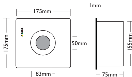
"CRYSTALITE" Cat. CE-SPC-1X3W-N
